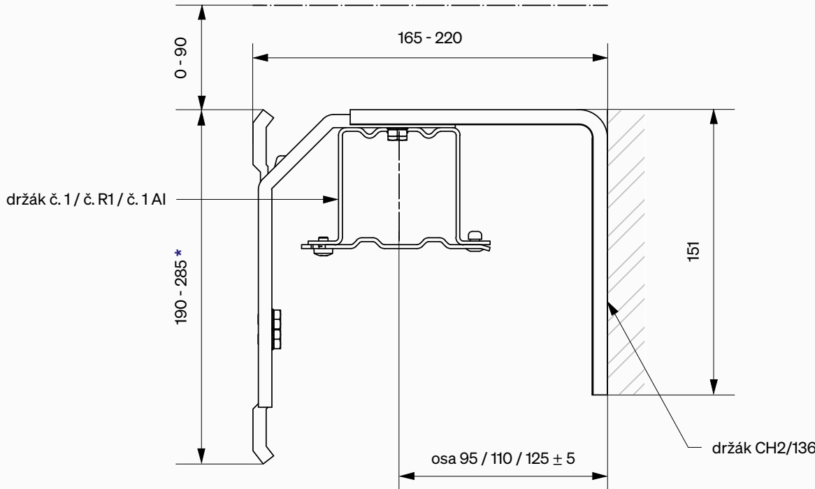
Držák CH3/136
