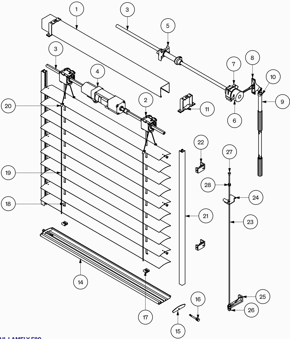
DETAIL LAMELY F80
